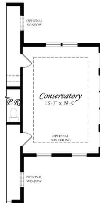
Opt. Conservatory
